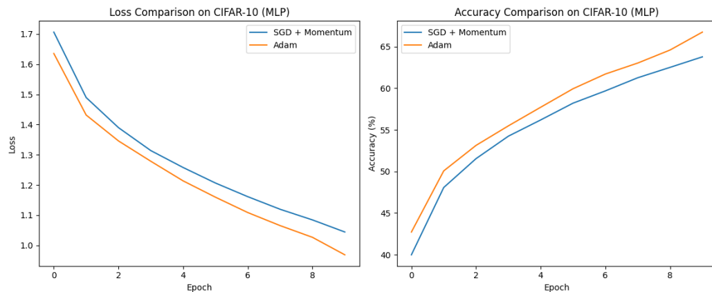
Loss and accuracy comparison: SGD + Momentum vs Adam
